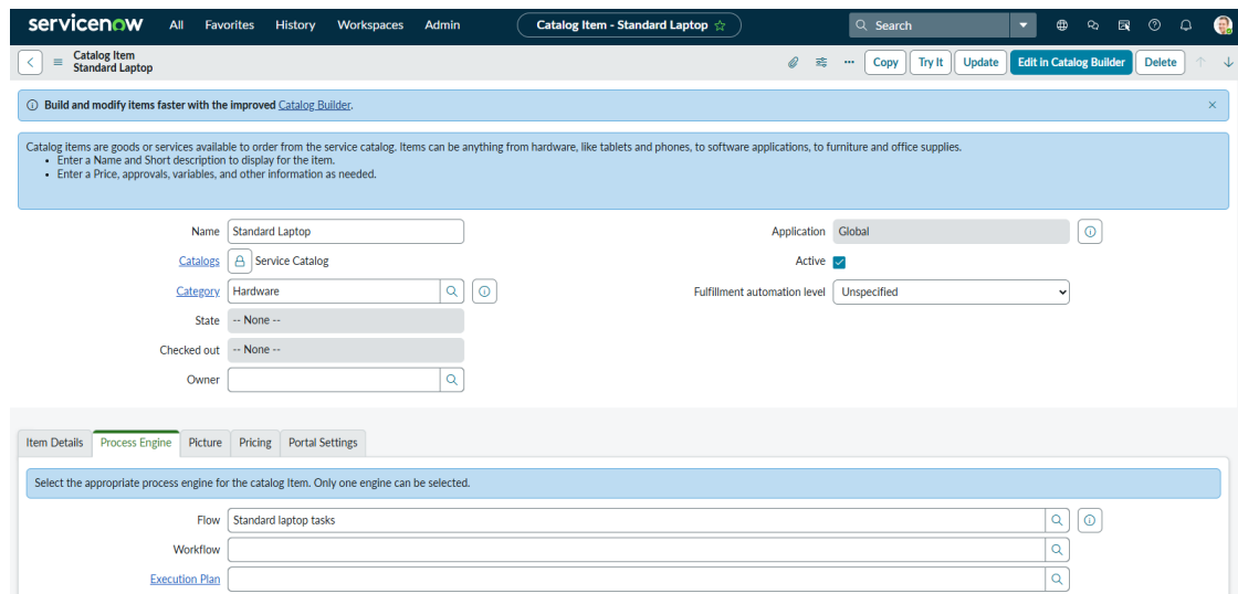
Figure 18: Catalog item form after the flow was linked
